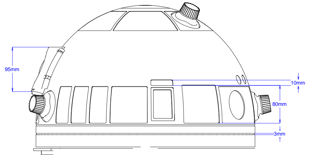
LEFT VIEW
